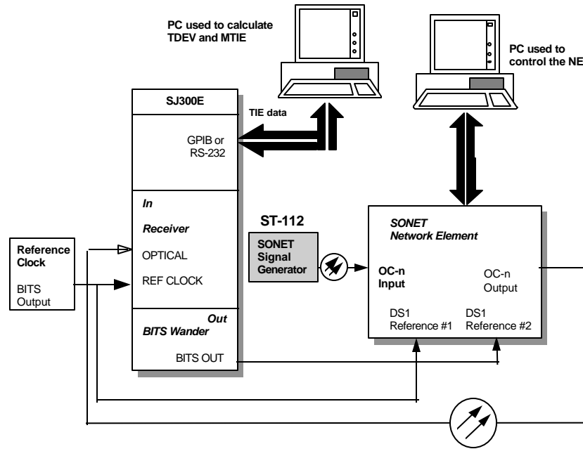
Figure 2-7. SONEC OC-N Phase Transient Specification conformance testing.
