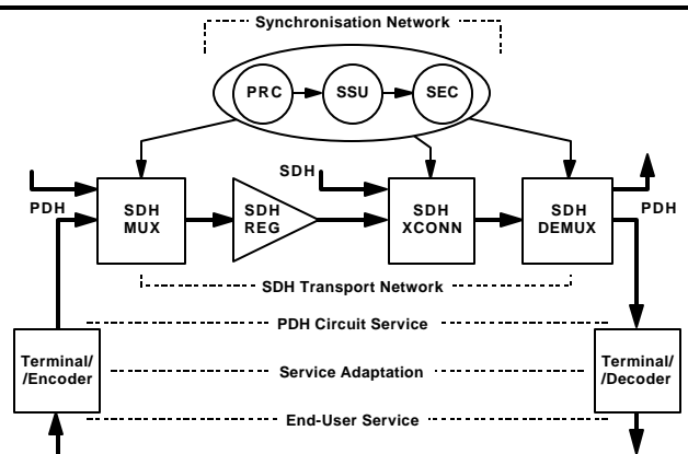
Figure 2-14. Reference broadband network
