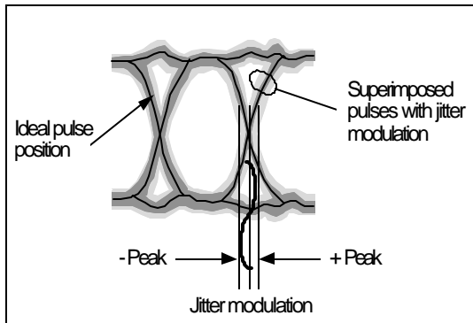
Figure 2-22. Jitter as viewed on an oscilloscope
